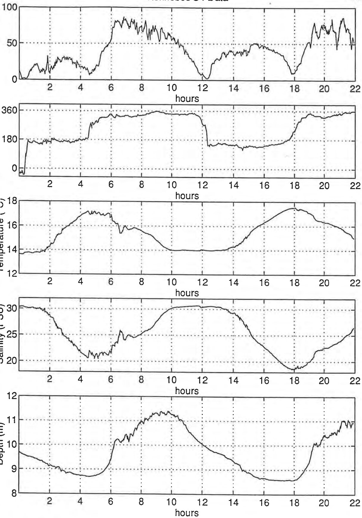
Figure D.6.1 Data from S4 moored 5m off bottom at Phippsburg, beginning 10:35, 9/1/94, ending 8:30, 9/2/94.
