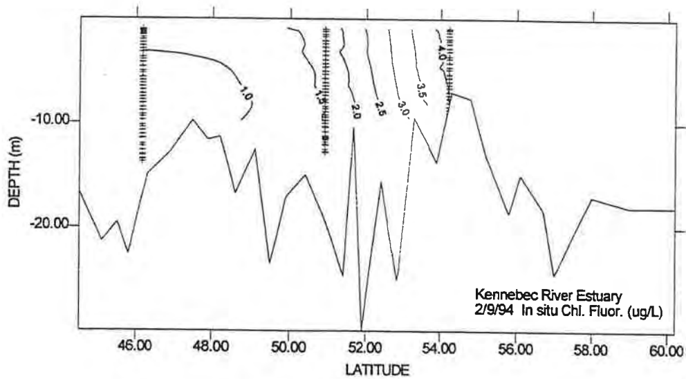
Figure A.2.4. Vertical section contour plots of in situ chlorophyll fluorescence (ug/L), from the mouth to the head, in the Damariscotta, Sheepscot and Kennebec River estuaries in February 1994. Latitude is given as minutes north of 43 degrees N. Sample depths are shown as crosses at each station.
