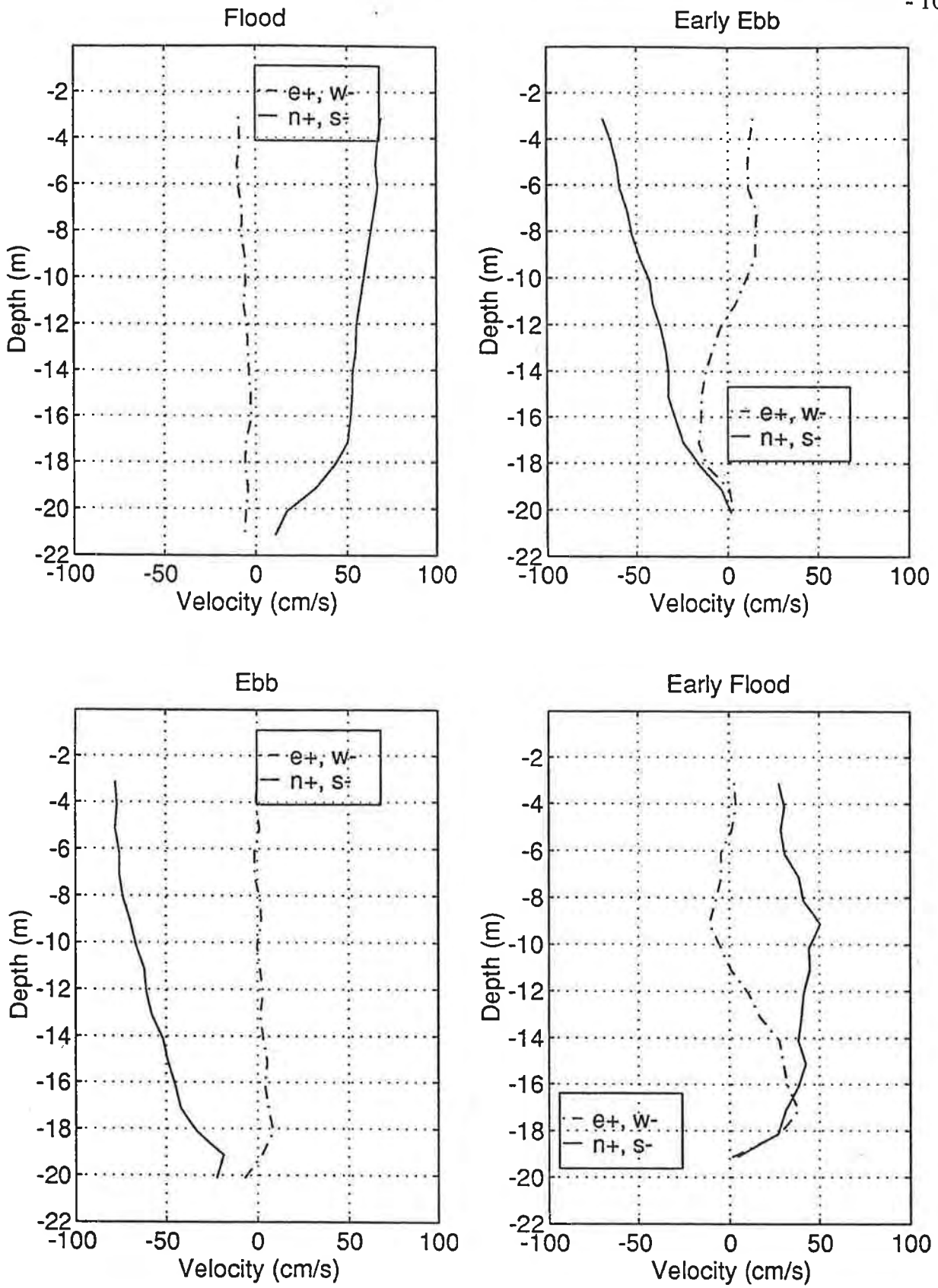
Figure C.7.3 (9/17/95) Velocity vs. Depth at Fish Plant
