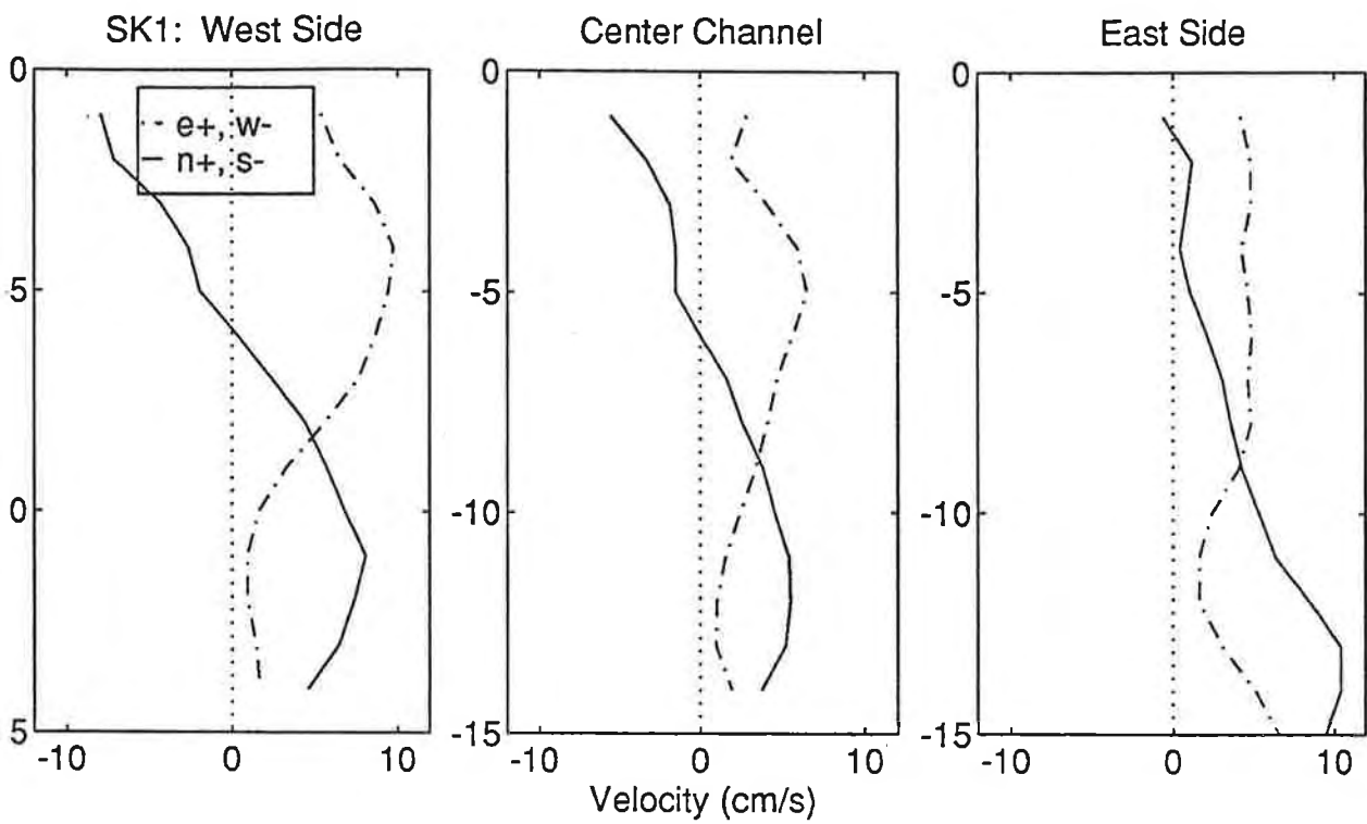
Figure C.6.2 (9/30/94) Tidal Mean Velocity v. Depth at Cox Head
