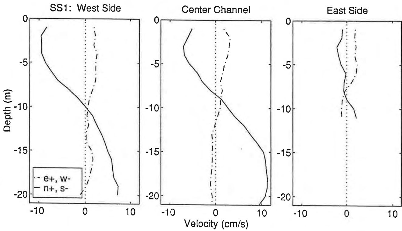
Figure C.6.6 (9/27/94) Tidal Mean Velocity v. Depth at Barbers Island
