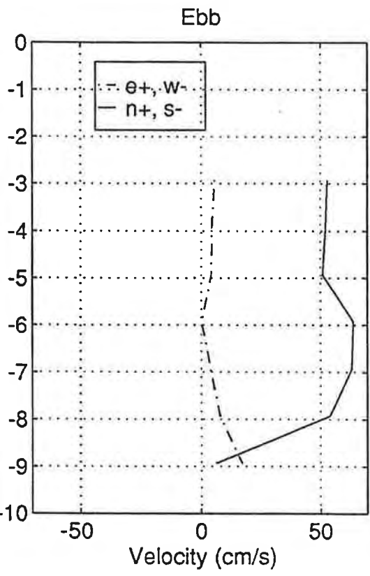
Figure C.7.5b (9/16/95) Velocity vs. Depth at Twing Point
