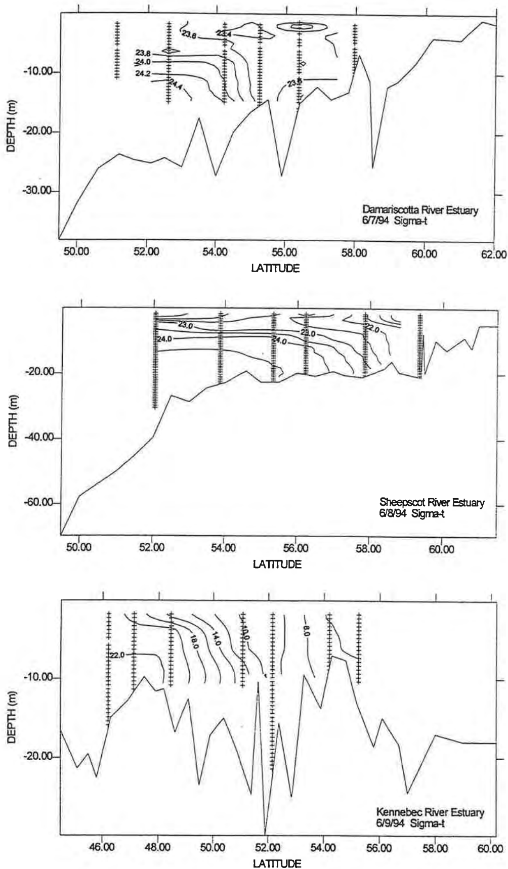
Figure A.4.3. Vertical section contour plots of Sigma-t, from the mouth to the head, in the Damariscotta, Sheepscot and Kennebec River estuaries in June 1994. Latitude is given as minutes north of 43 degrees N. Sample depths are shown as crosses at each station.
