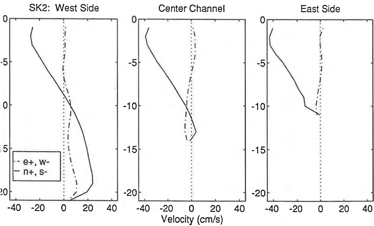
Figure C.6.3 (9/30/94) Tidal Mean Velocity v. Depth at Phippsburg
