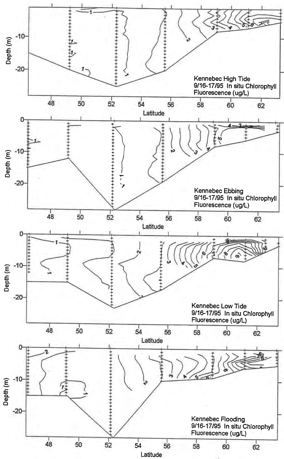
Figure A.7.4 Vertical section contour plots of in situ chlorophyll fluorescence (ug/L), from the mouth to the head, in the Kennebec River estuary at 3 hour intervals on September 16-17, 1995. Latitude is in minutes north of 43 degrees N. Sample depths are shown as crosses at each station.
