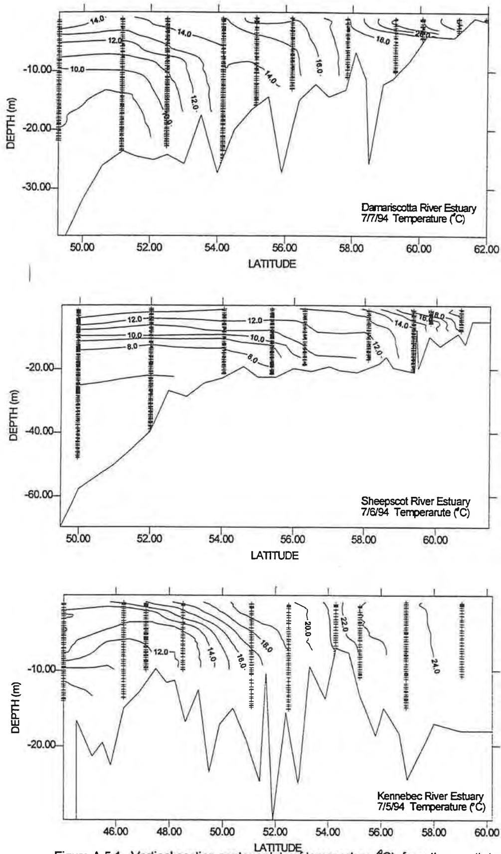
Figure A.5.1. Vertical section contour plots of temperature ( ^{\circ}\text{C} ), from the mouth to the head, in the Damariscotta, Sheepscot and Kennebec River estuaries in July 1994. Latitude is given as minutes north of 43 degrees N. Sample depths are shown as crosses at each station.
