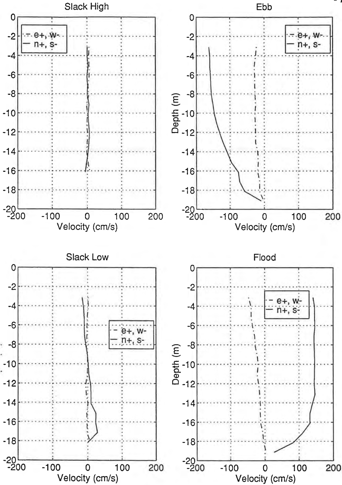
Figure C.7.4 (9/16/95) Velocity vs. Depth at Chops Point
