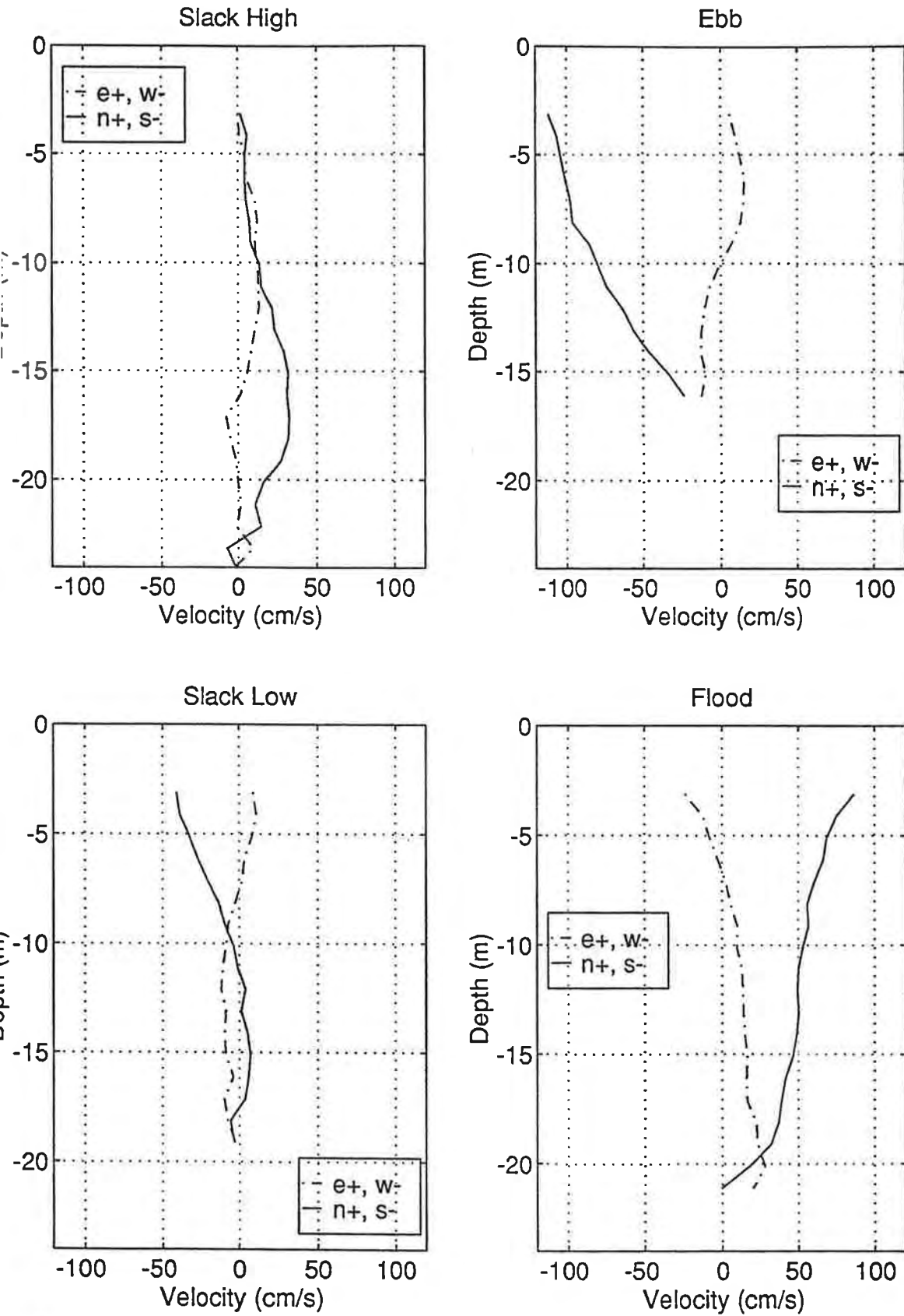
Figure C.7.1 (9/17/95) Velocity vs. Depth at Phippsburg
