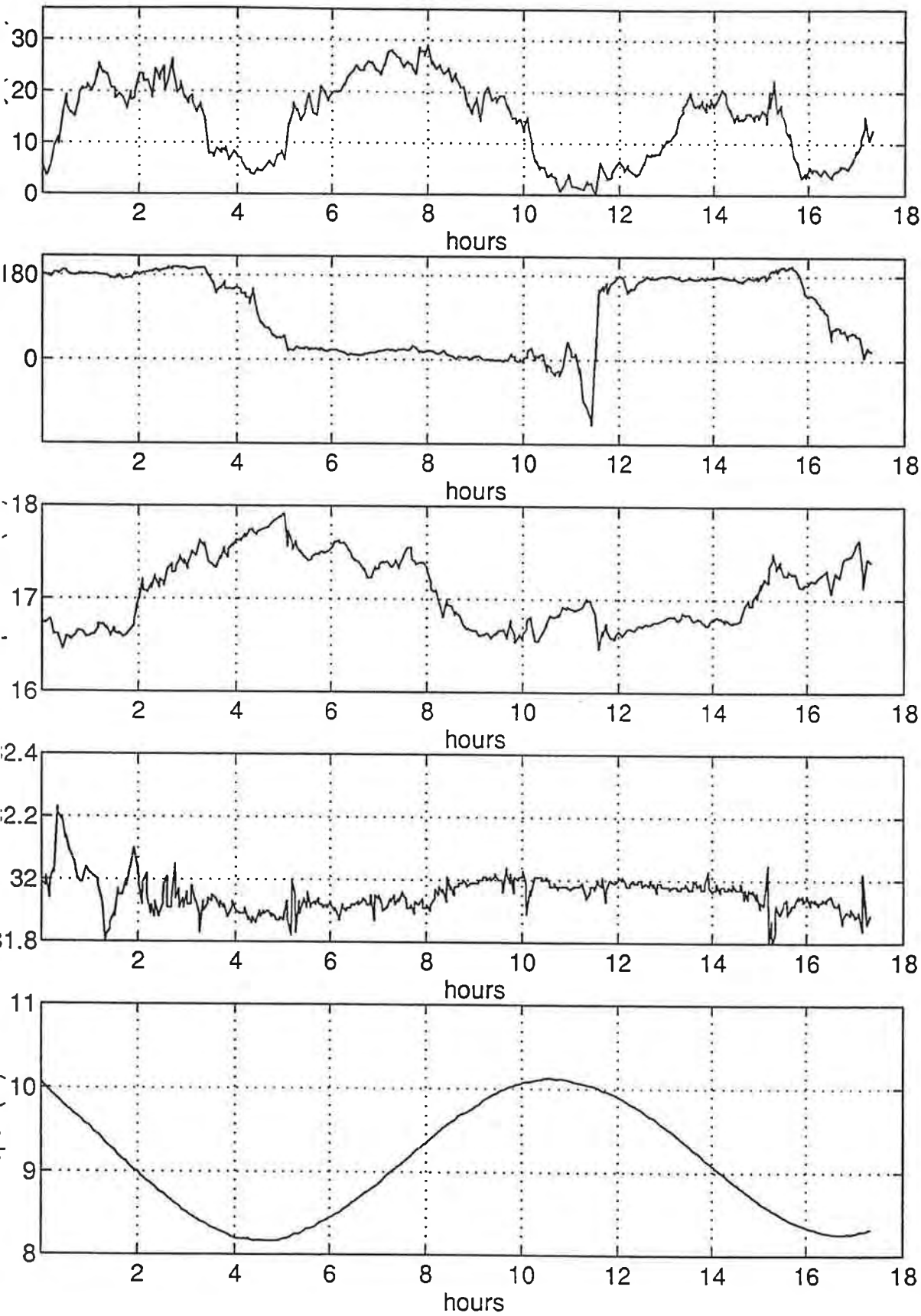
Figure D.6.3 Data from S4 moored 5m off the bottom at Wentworth Point, beginning 19:30, 8/29/94, ending 12:45, 8/30/94.
