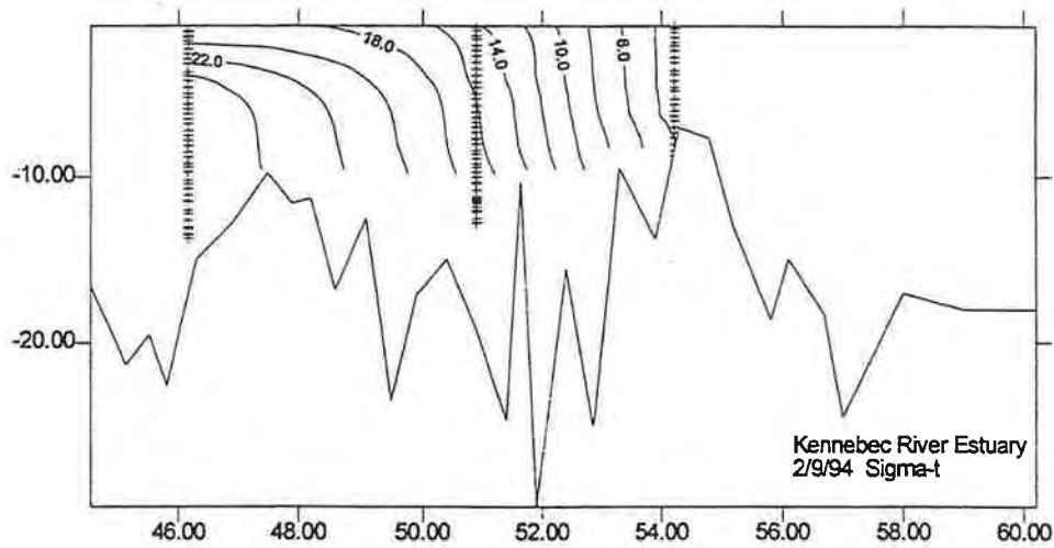
Figure A.2.3. Vertical section contour plots of Sigma-t, from the mouth to the head, in the Damariscotta, Sheepscot and Kennebec River estuaries in February 1994. Latitude is given as minutes north of 43 degrees N. Sample depths are shown as crosses at each station.
