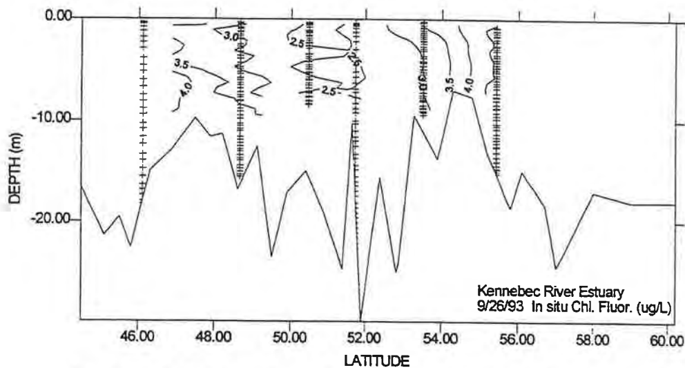
Figure A.1.4. Vertical section contour plots of in situ chlorophyll fluorescence (ug/L), from the mouth to the head, in the Damariscotta, Sheepscot and Kennebec River estuaries in September 1993. Latitude is given as minutes north of 43 degrees N. Sample depths are shown as crosses at each station.
