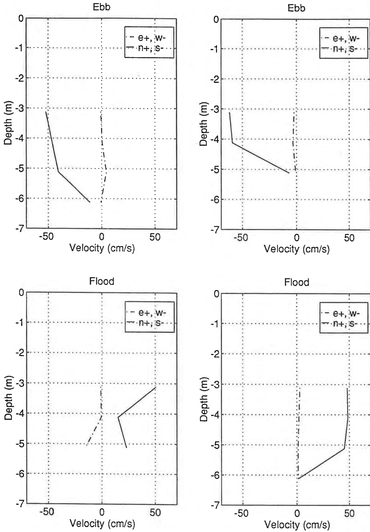
Figure C.7.6 (9/16/95) Velocity vs. Depth at Green Point
