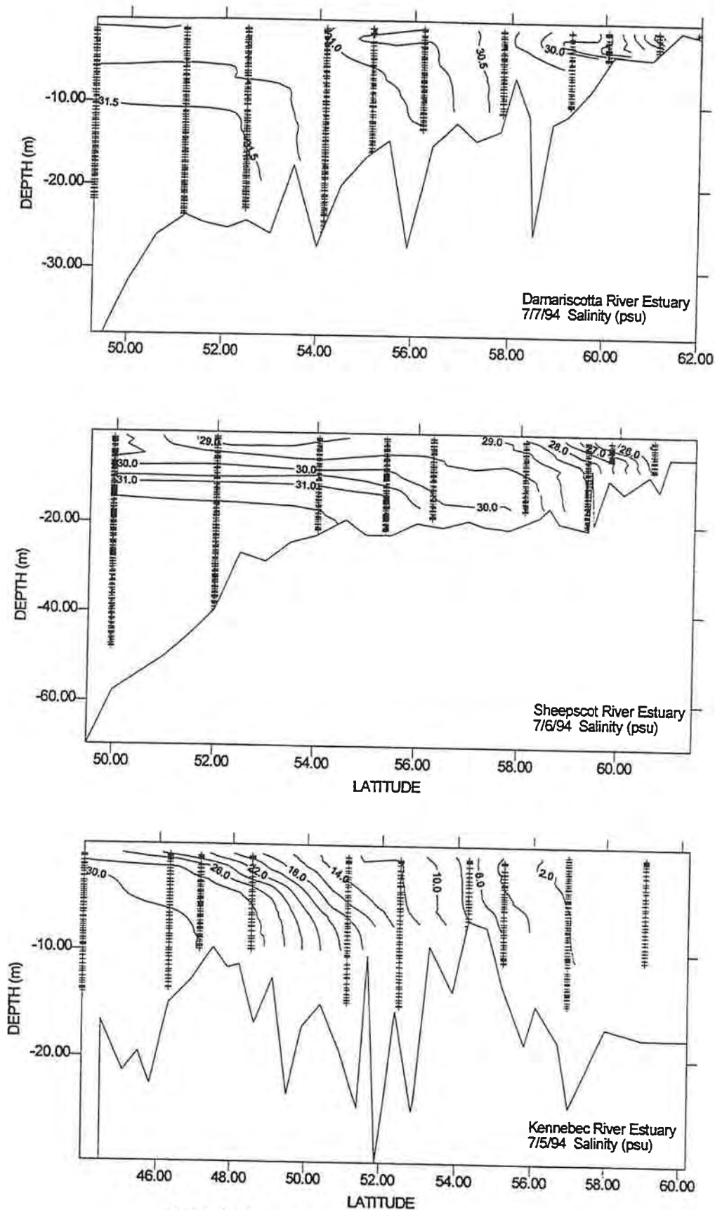
Figure A.5.2. Vertical section contour plots of salinity (psu), from the mouth to the head, in the Damariscotta, Sheepscot and Kennebec River estuaries in July 1994. Latitude is given as minutes north of 43 degrees N. Sample depths are shown as crosses at each station.
