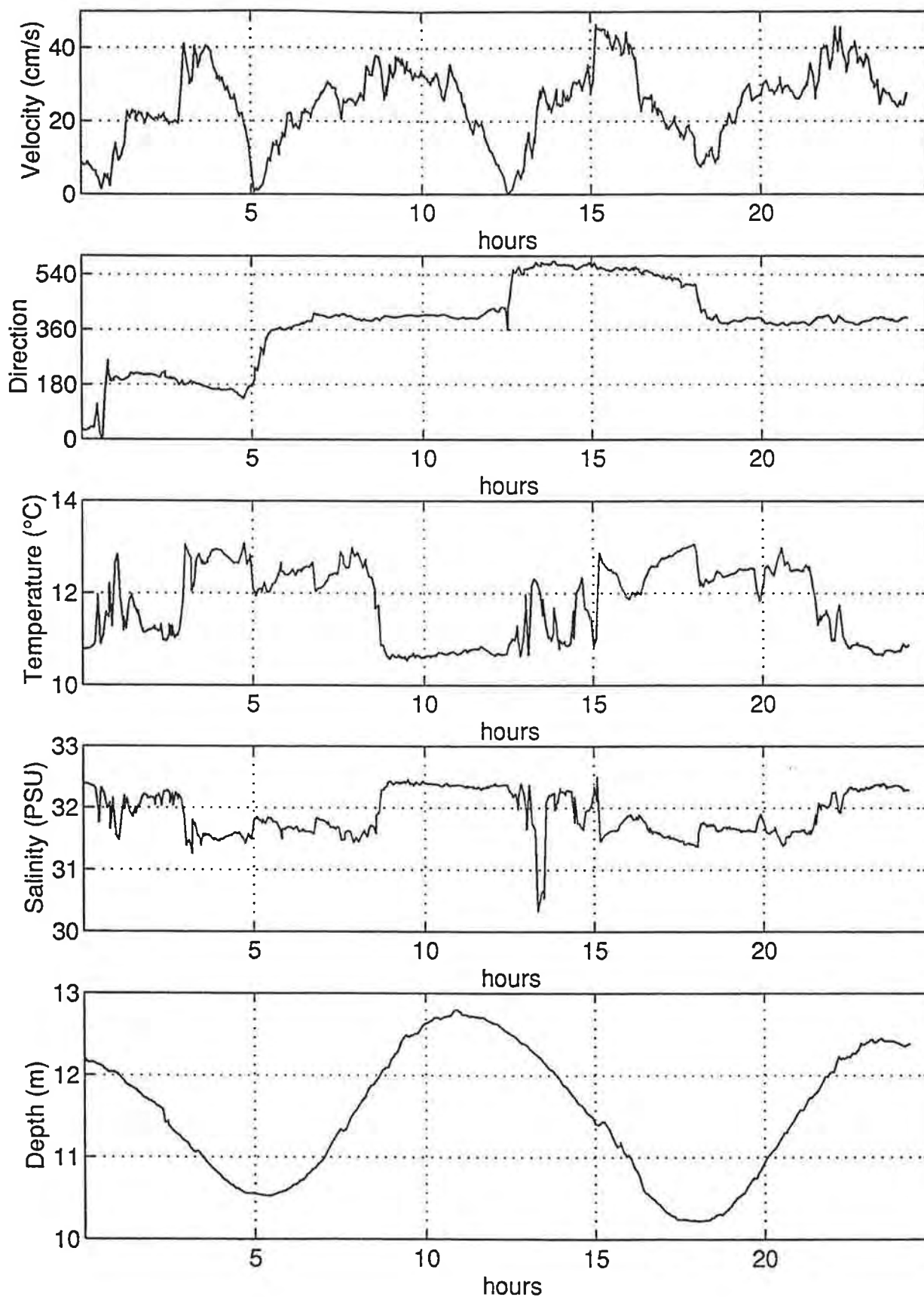
Figure D.6.2 Data from S4 moored 5m off the bottom off Barbers Island, beginning 7:55, 8/31/94, ending 8:15, 9/1/94.
