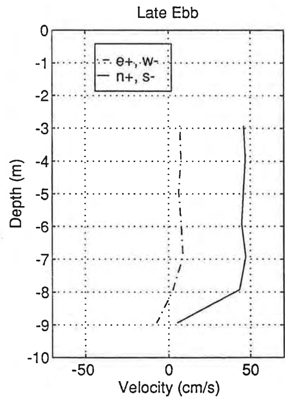
Figure C.7.5b (9/16/95) Velocity vs. Depth at Twing Point
