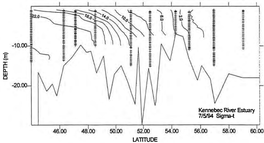
Figure A.5.3. Vertical section contour plots of sigma-t, from the mouth to the head, in the Damariscotta, Sheepscot and Kennebec River estuaries in July 1994. Latitude is given as minutes north of 43 degrees N. Sample depths are shown as crosses at each station.
