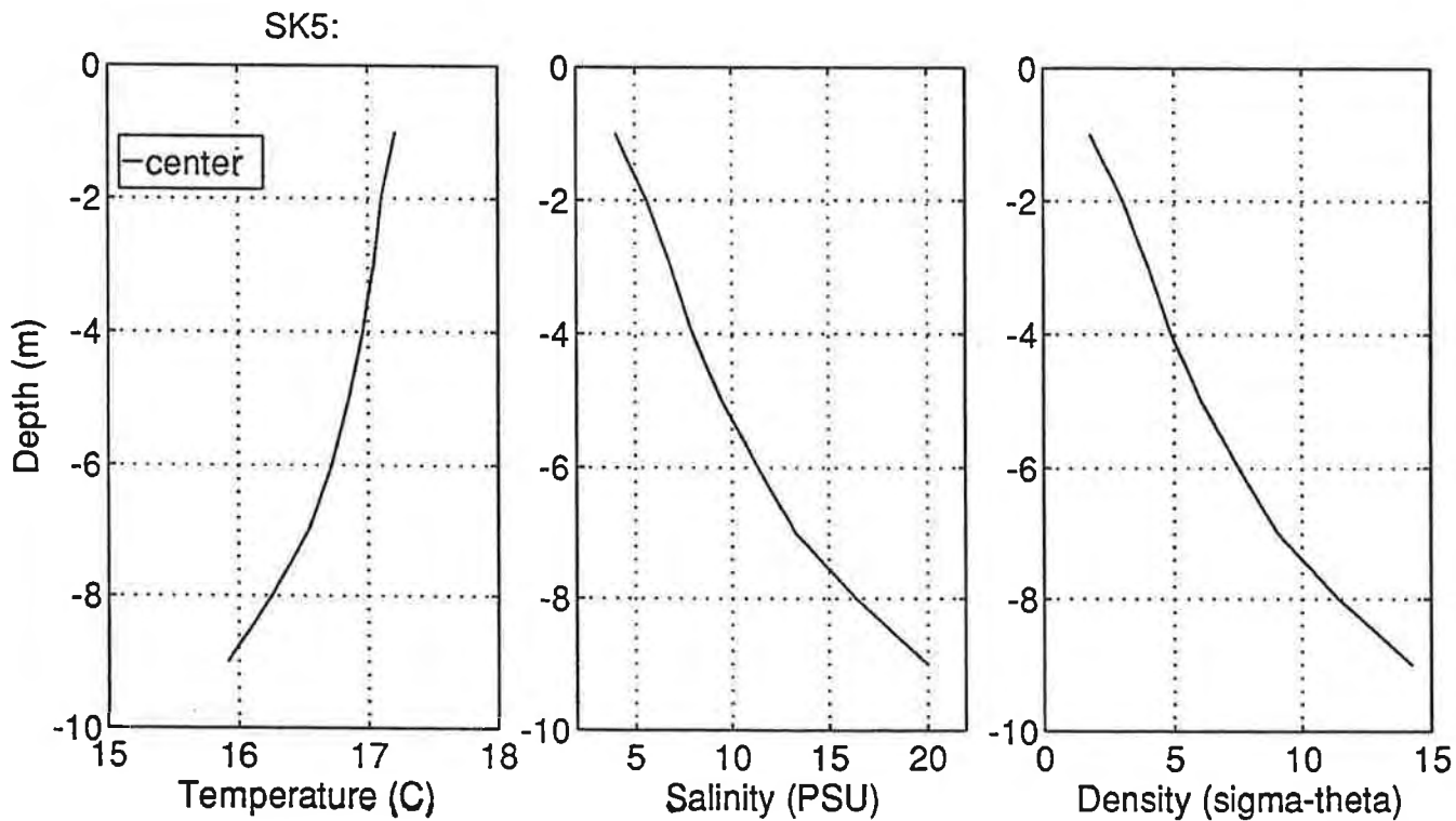
Figure B.6.1 (9/29/94) Tidal Mean Hydrography v. Depth at Sasanoa River
