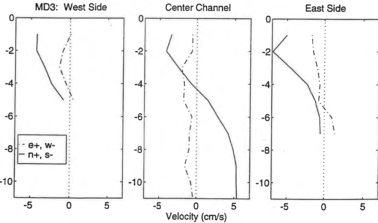
Figure C.3.4 (5/4/94) Tidal Mean Velocity v. Depth at Dodge Point
