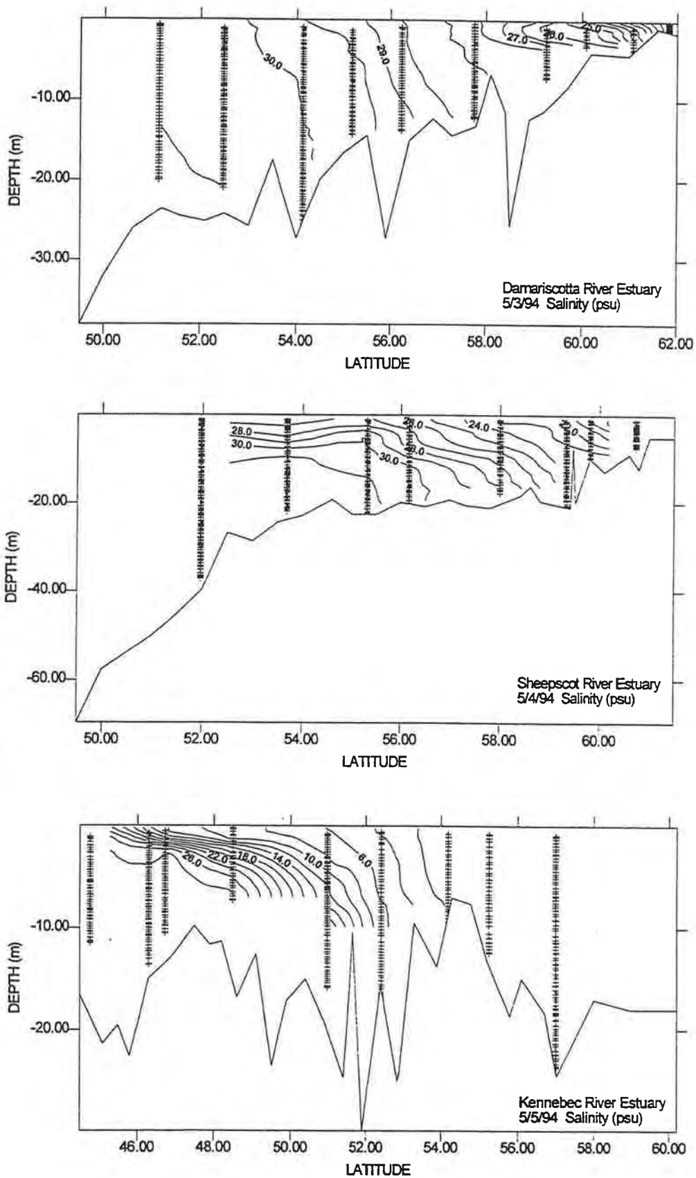
Figure A.3.2. Vertical section contour plots of salinity (psu), from the mouth to the head, in Damariscotta, Sheepscot and Kennebec River estuaries in May 1994. Latitude is given as minutes north of 43 degrees N. Sample depths are shown as crosses at each station.
