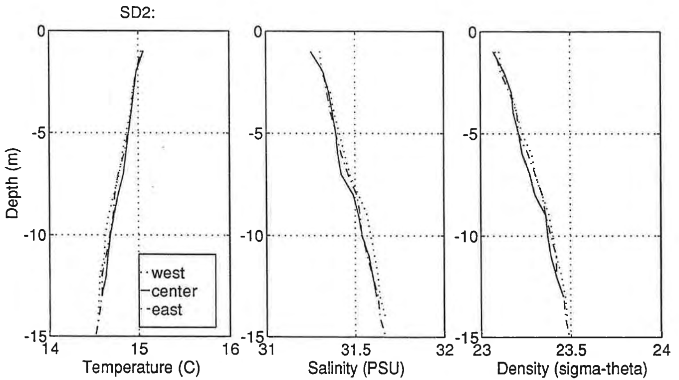
Figure B.6.9 (9/26/94) Tidal Mean Hydrography v. Depth at Wentworth Point
