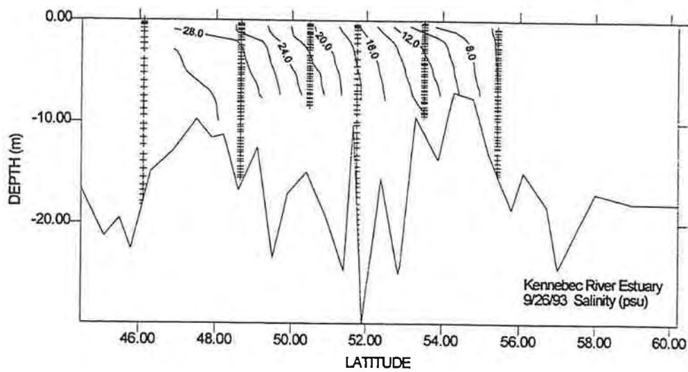
Figure A.1.2. Vertical section contour plots of salinity (psu), from the mouth to the head, in the Damariscotta, Sheepscot and Kennebec River estuaries in September 1993. Latitude is given as minutes north of 43 degrees N. Sample depths are shown as crosses at each station.
